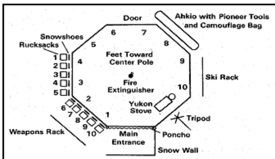
Figure 7-3. Ten-man tent.
