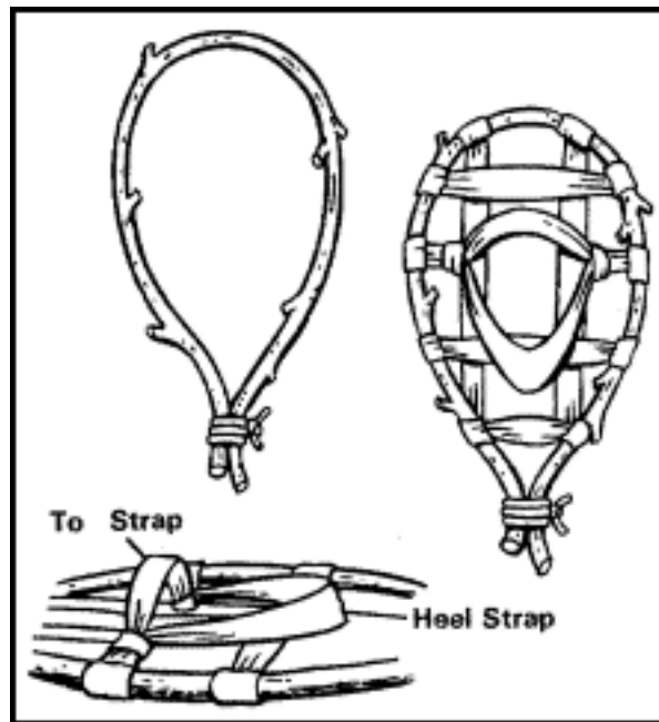
Figure 8-2. Improved snowshoes.
