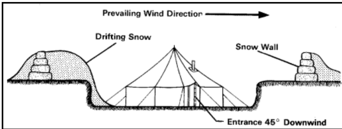
Figure 3-2. Windbreak.
