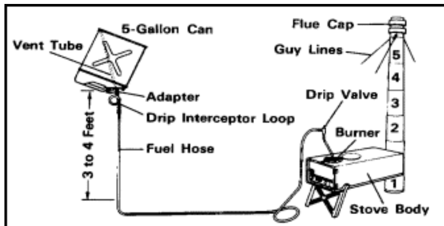
Figure 3-4. Yukon stove.
