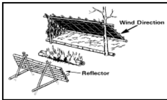
Figure 10-3. Single lean-to.
