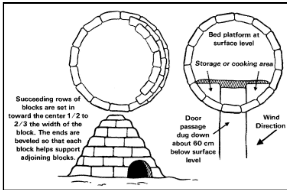
Figure 10-9. Snow house.
