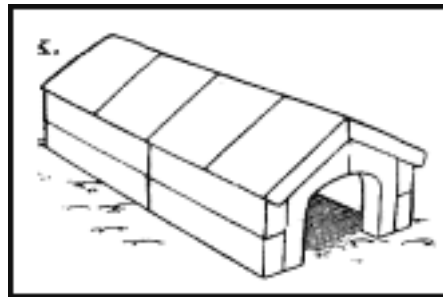
Figure 10-8. Individual snow house.
