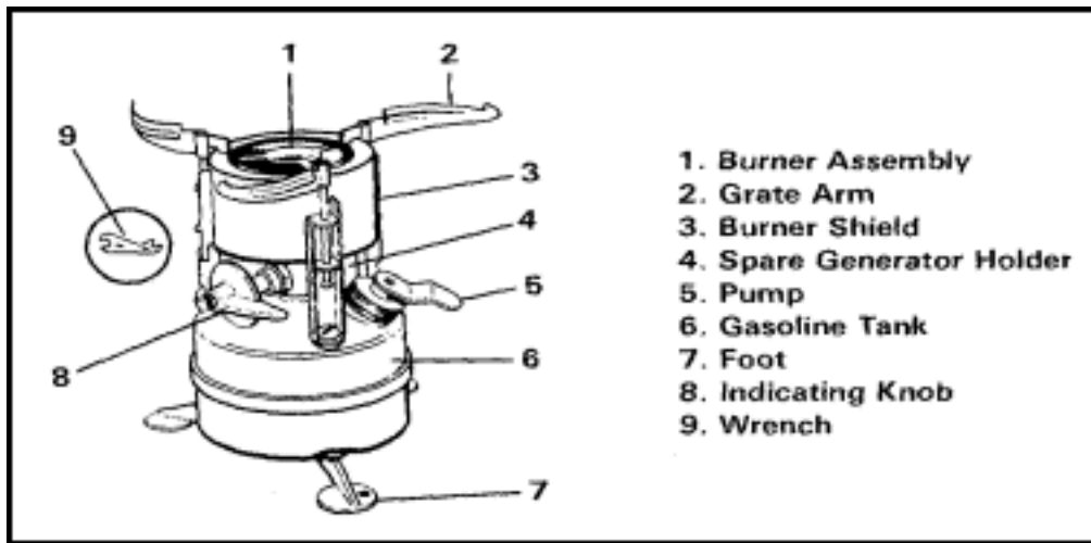
Figure 3-6. Gasoline cooking stove, M1950.
