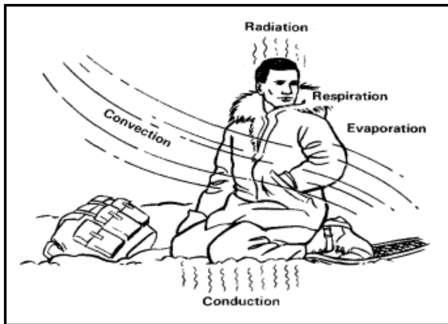
Figure 6-1. Mechanisms of heat loss from the body.
