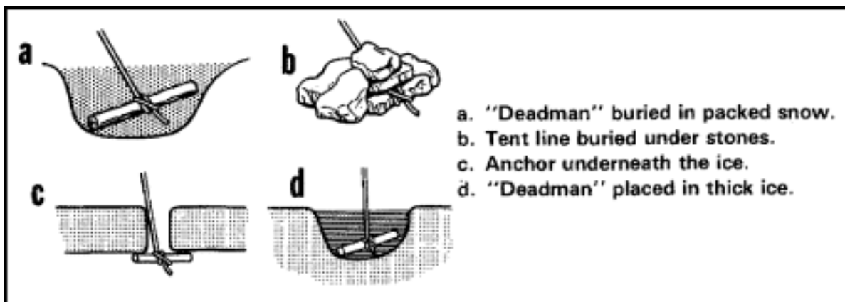
Figure 3-3. Deadmen.
