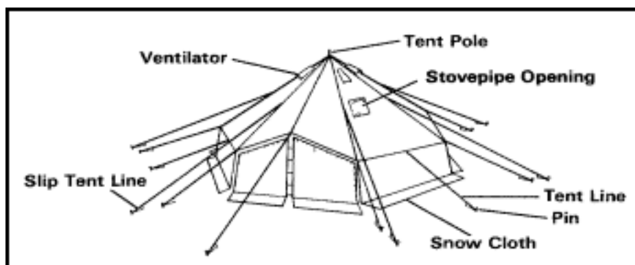
Figure 3-1. Ten-man arctic tent.
